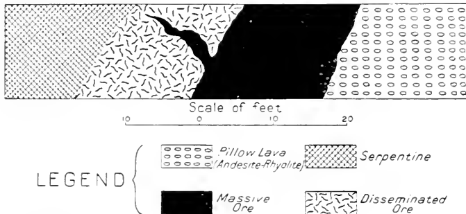
Cross-section at the Alexo nickel mine, on the 120-foot level, Dundonald and Clergue Townships, Timiskaming District, Ontario. The massive ore cuts through the disseminated ore, and was deposited at a later period in the history of the ore body than the disseminated ore. This age relation between the massive and disseminated ore is also shown in the two preceding cross-sections.
